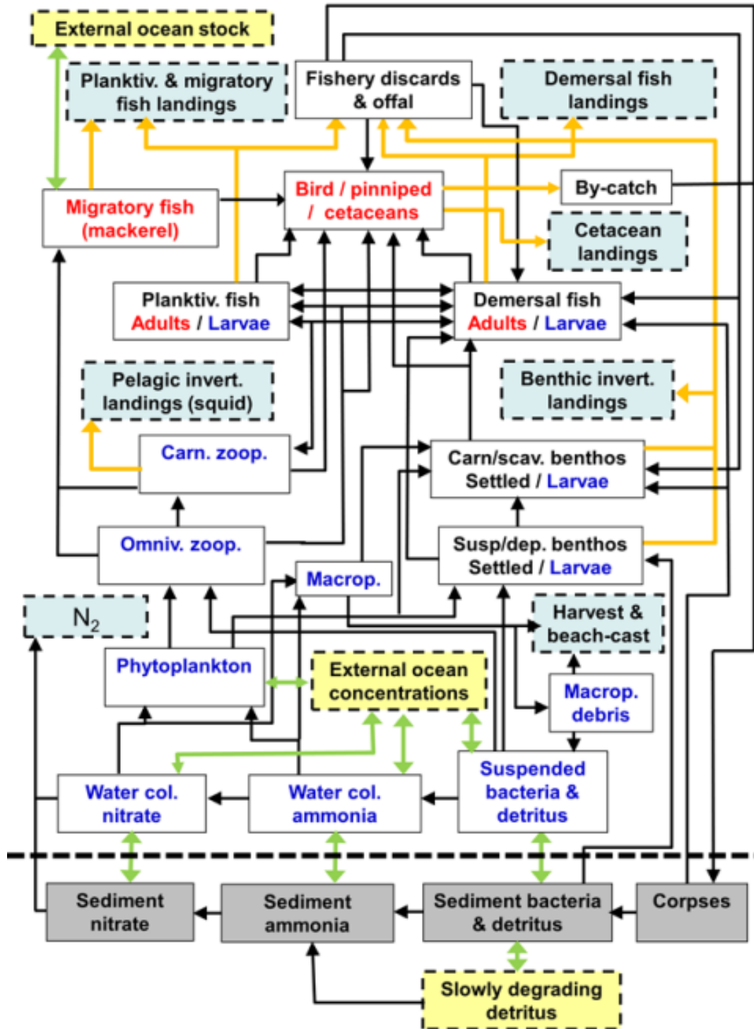
TO BE UPDATED WITH ADDITION OF ICE NUTRIENTS, DETRITUS AND ALGAE, AND MARITIME MAMMALS. FIGURE 1. Schematic of the food web compartments of the StrathE2E2 model. Green arrows represent advection, mixing and migration; orange arrows represent fishery-related fluxes; black arrows represent biological fluxes. Red labelled components are active migrators whilst blue are subject to passive advection and mixing and black are anchored. Pale blue boxes represent quantities that are exported from the model whilst yellow are imported. The model also includes fluxes from living components to ammonia, detritus and corpses due to excretion, defecation and death but these are not shown for clarity. Also for clarity, birds, pinnipeds and cetaceans are combined as a single
