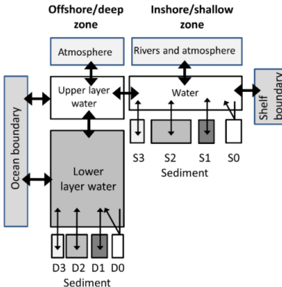
TO BE UPDATED TO ILLUSTRATE SEA ICE COMPARTMENTS. FIGURE 2. Schematic showing the horizontal and vertical spatial structure of the model. The compartments
