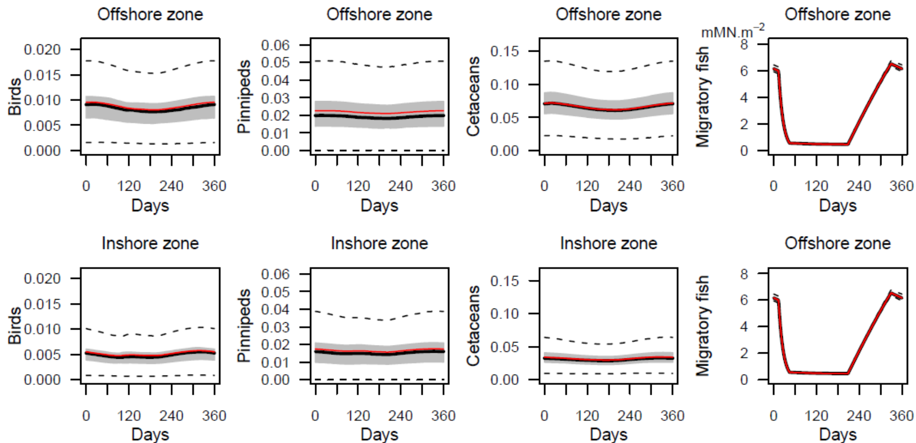
FIGURE 20 Stationary annual cycles of the birds & mammals guilds, migratory fish, and dead corpses for the 1970-1999 fitted model. Dashed lines span the 99% likelihood interval of model outputs given the observed indices of the state of the North Sea during this period. Grey shading spans the 50% likelihood interval. Solid black line is the median of the likelihood distribution and the red line is the maximum likelihood model. Columns of panels are different variables output from the model, rows are different spatial compartments. Units for all variables: \text{mMN.m}^{-2} .
