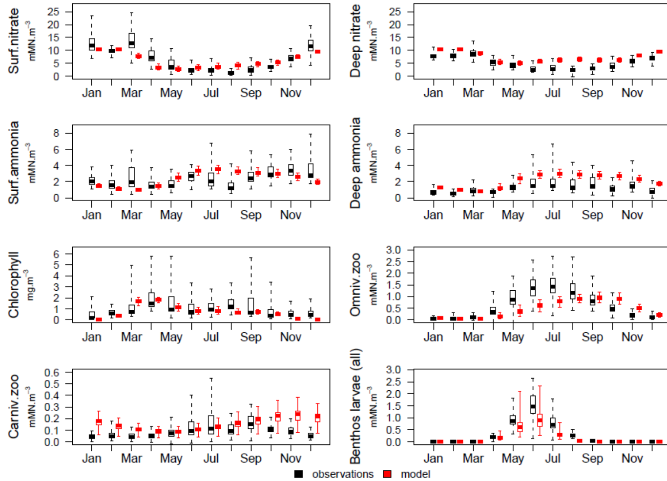
FIGURE 24 Monthly averages of the 1970-1999 stationary annual cycle daily resolution output for the whole model domain (red) and observed monthly averaged data from the North Sea (black). Box and whiskers for the model data show the 0.5, 25, 50, 75 and 99.5 centiles of the likelihood distribution of results given the uncertainty in fitted parameter values. For the observed data the box and whiskers show the equivalent variability in measurements from the North Sea aggregated over the period 1970-1999. Note that the model was not fitted to these observed data so the comparison represents a validation of the fitted model.
